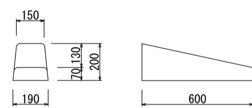
切下げ部7cm (33kg)
