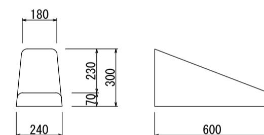
切下げ部7cm (55kg)
