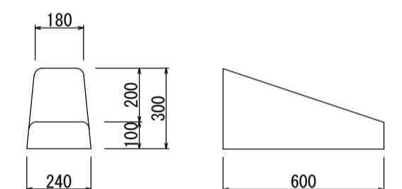
切下げ部10cm (60kg)
