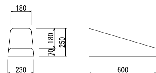
切下げ部7cm (47kg)
