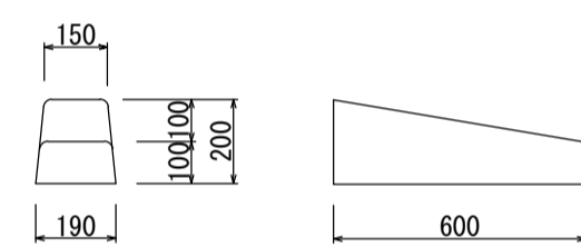
切下げ部10cm (33kg)
